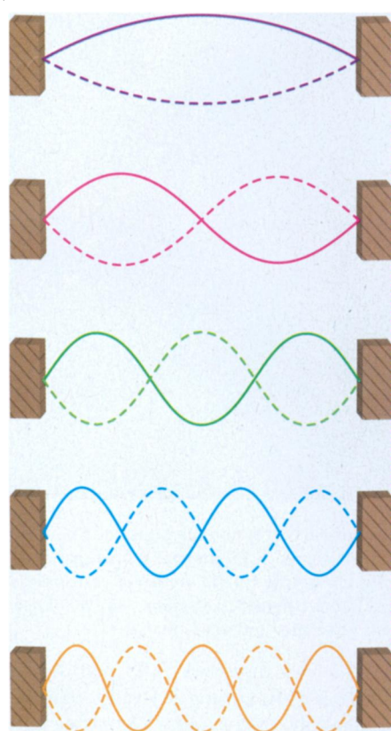
Figure 3. Fermi, Pasta and Ulam expected the energy in their mass-spring system eventually to become shared equally between different modes of motion, which are analogous to the modes of vibration of a plucked violin string. The fundamental mode of vibration for such a string (purple) corresponds to the note that is heard. Higher-frequency vibrational modes give rise to various harmonics of that note. The motions shown here correspond to the second (pink), third (green), fourth (blue) and fifth (orange) harmonics.
